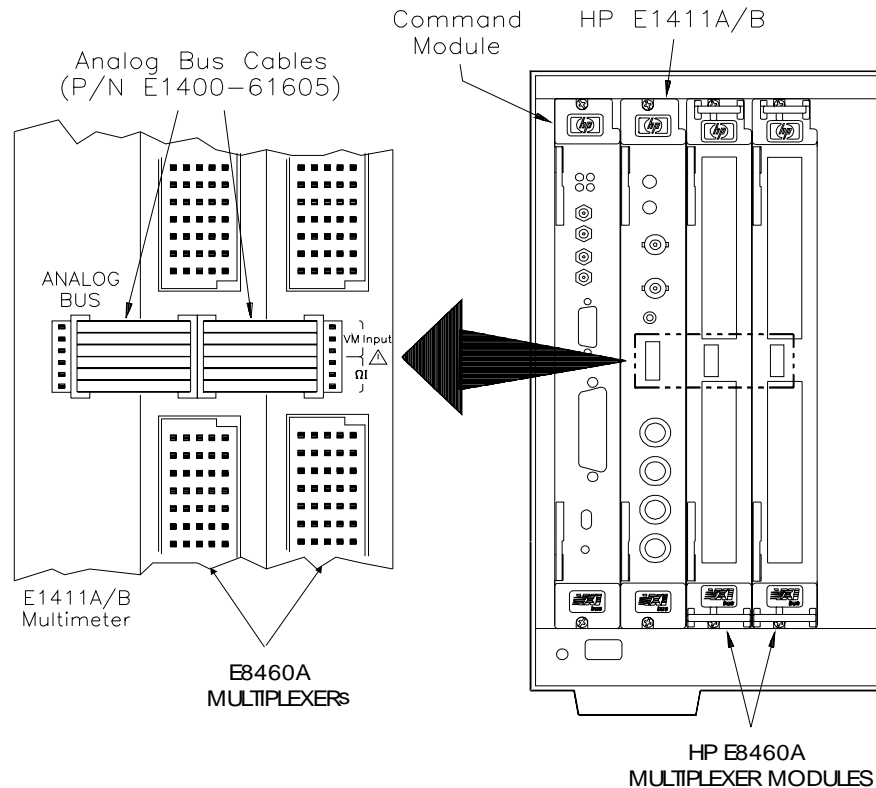
Figure 1-9. HP E1411A/B Connections to the Analog Bus
