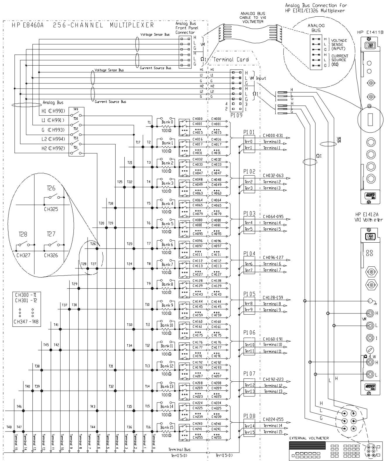
Figure 1-1. HP E8460A Simplified Schematic
